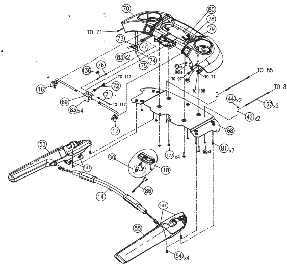
Detail view of Console Base
