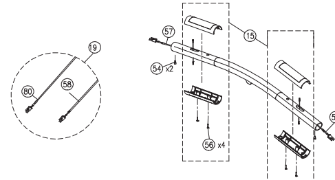
Detail view of Crossbar
