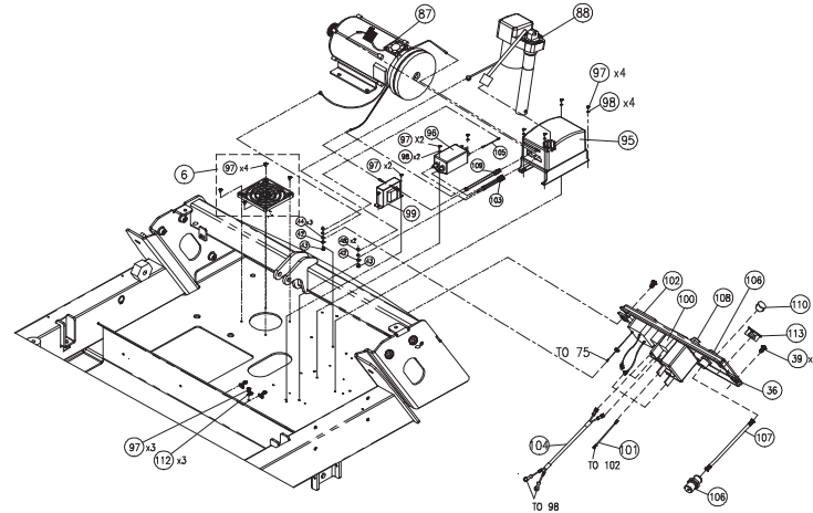
Detail View of Electrical Components
