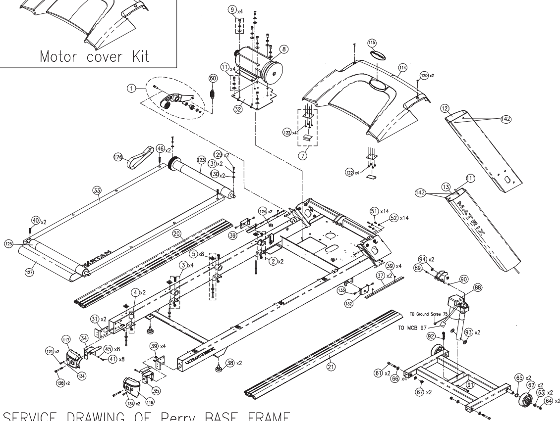
SERVICE DRAWING OF Perry BASE FRAME
